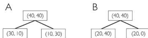
Figure 3.20: Decision tree data splits
