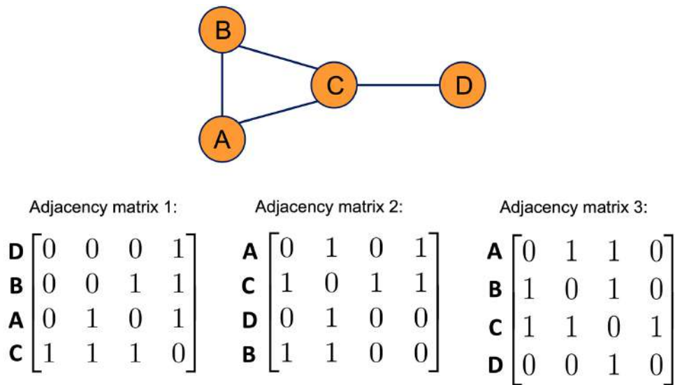
Figure 18.5: Different adjacency matrices representing the same graph
