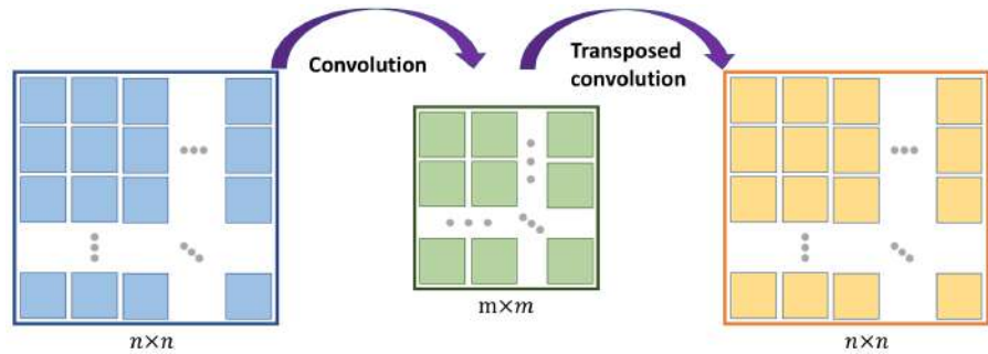
Figure 17.12: Transposed convolution
