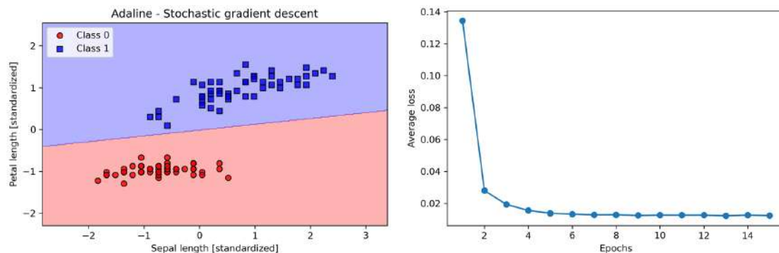
Figure 2.15: Decision regions and average loss plots after training an Adaline model using SGD
