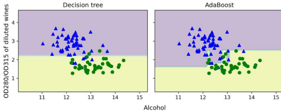
Figure 7.11: The decision boundaries of the decision tree versus AdaBoost
